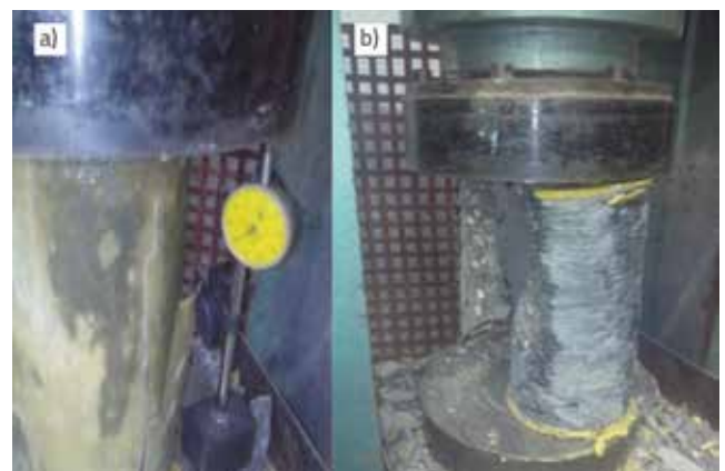
Figure 19. Failure modes and patterns of tested specimens: a) GFRP confined; b) CFRP confined
