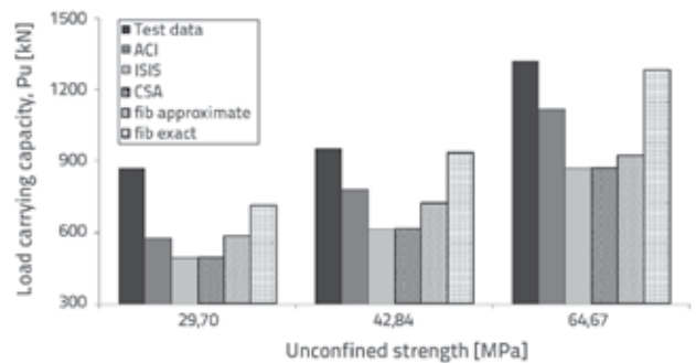
Figure 18. Comparison of test data and theoretical ultimate load carrying capacities of CFRP
