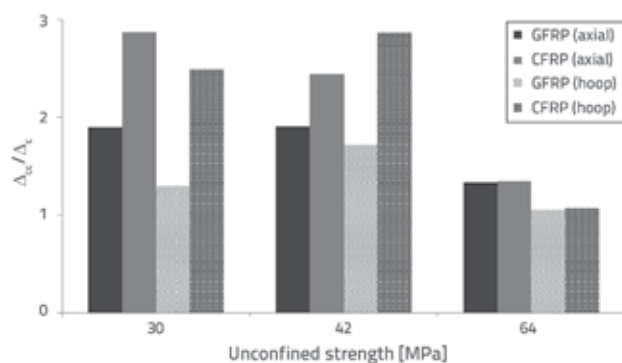
Figure 14. Comparison of energy absorption by confined specimens
